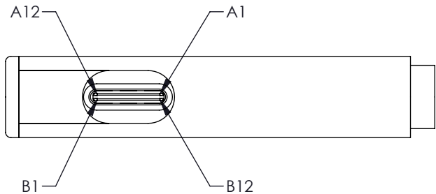
"P2" USB-C MALE
